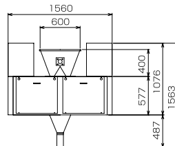
4 heads
